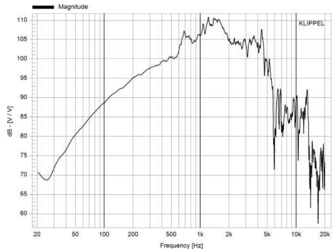
Frequency response measured with quasi-infinite baffle
