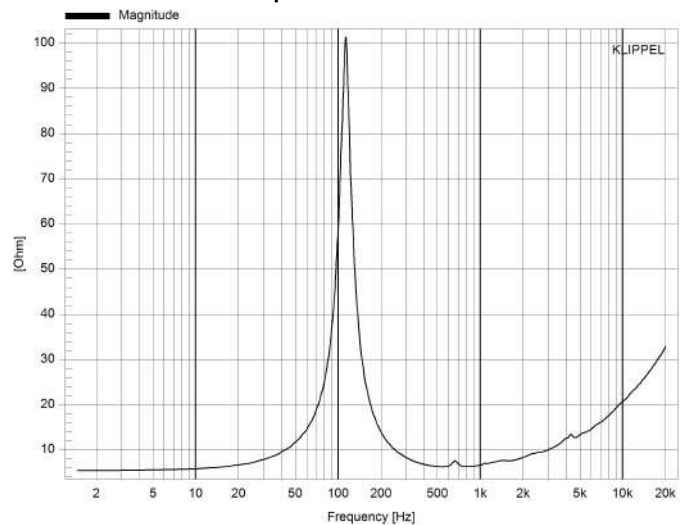
Impedance for 8Ω driver
